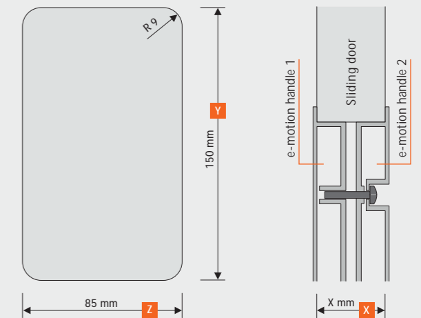
Typ L special+ (Handle on both sides mounted)
